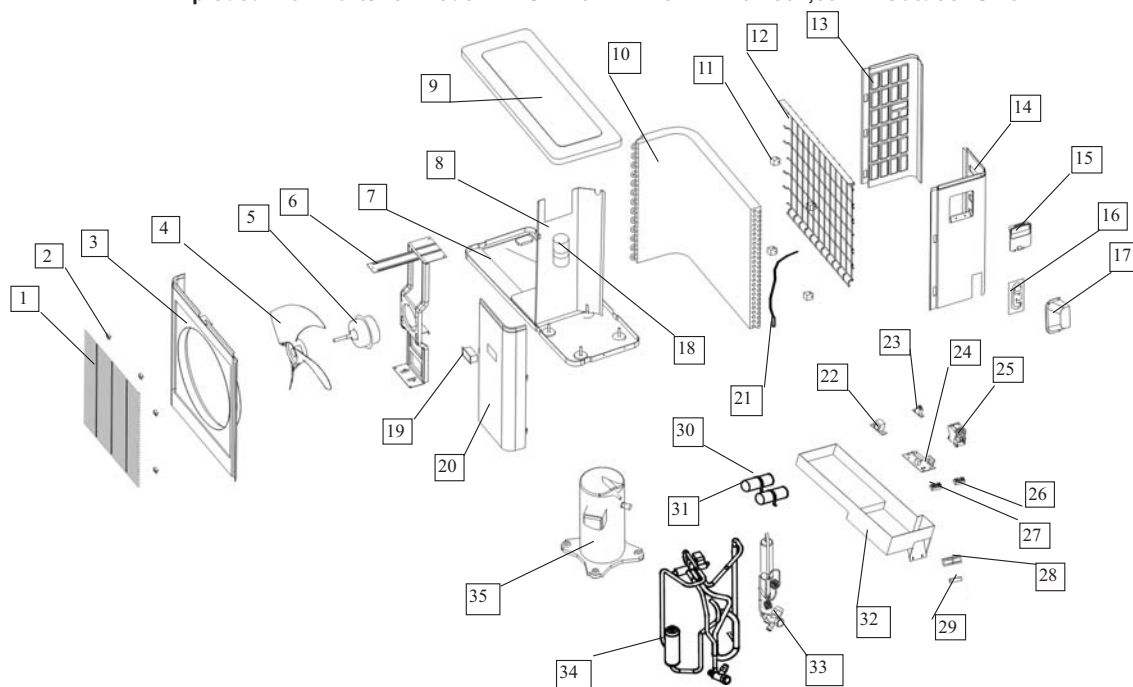
Exploded View Parts for Model KSWM024-H213 220-230V,60Hz : Outdoor Unit
