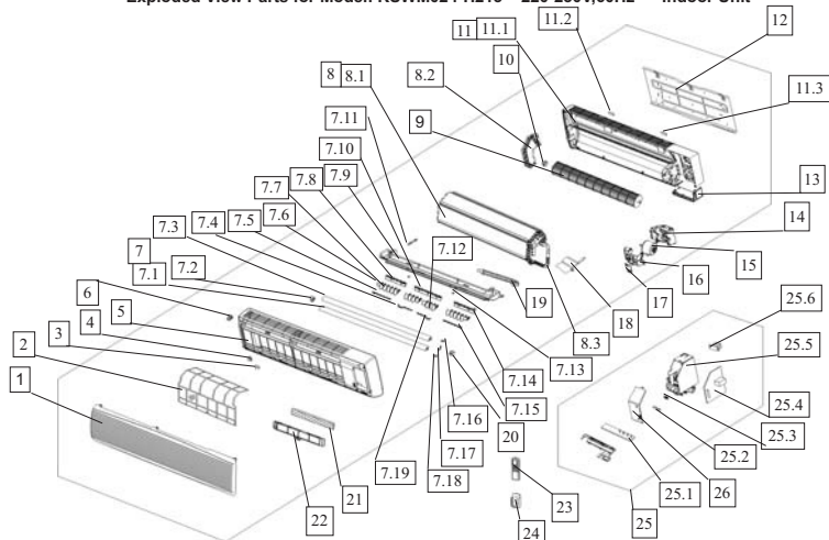
Exploded View Parts for Model: KSWM024-H213 220-230V,60Hz Indoor Unit
